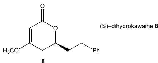
Figure 16 Structure de la (S)-dihydrokawaine 8
