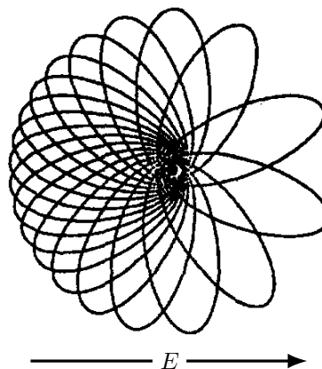
Precession of a nearly Keplerian elliptical orbit of the Rydberg electron about a positively charged nucleus in an electric field E = 1000 \text{ V} \cdot \text{cm}^{-1}
