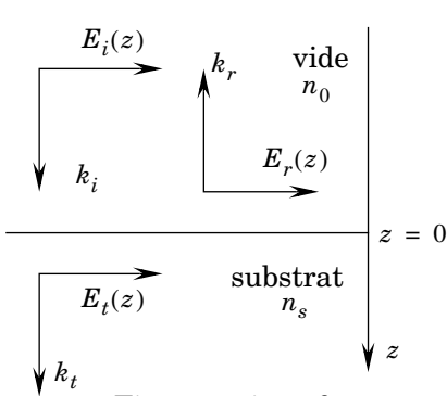
Figure 7 : interface vide/substrat
