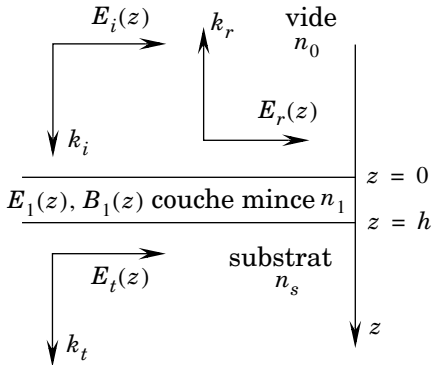
Figure 8 : structure substrat/couche mince/vide
