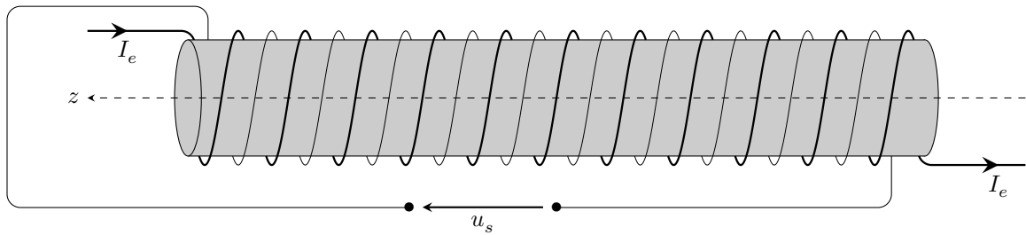
Figure 11 Fluxgate
