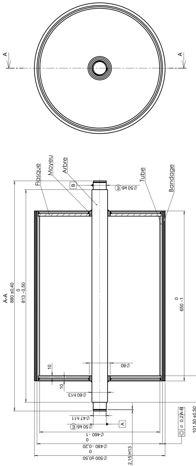
Figure 19 Rouleau 10
